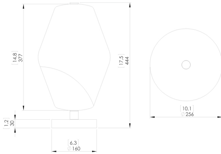
Dimensions in mm [inches]
