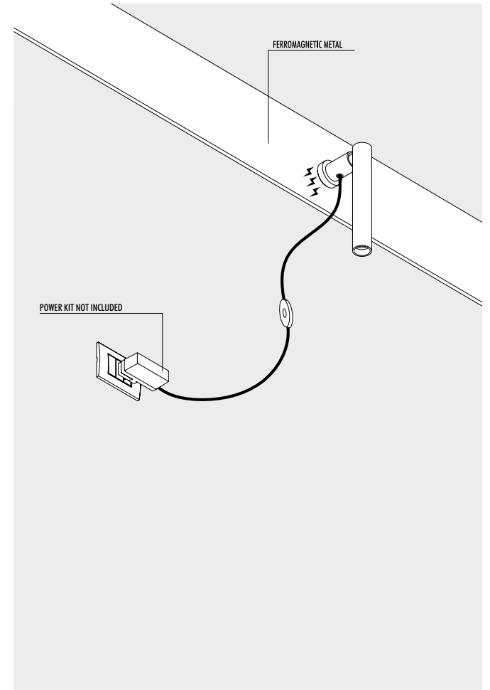
1A3180300.00.06 / 1A3180400.00.06 - MIRA MAGNETIC INSTALLATION WITH POWER SUPPLY KIT
